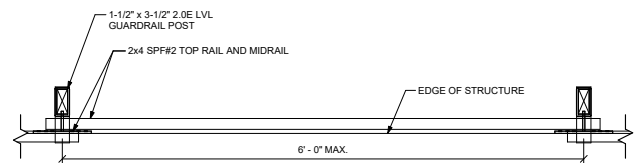
11 MIGHTYRAIL VERTICAL MOUNT EXAMPLE PLAN VIEW S101.2
