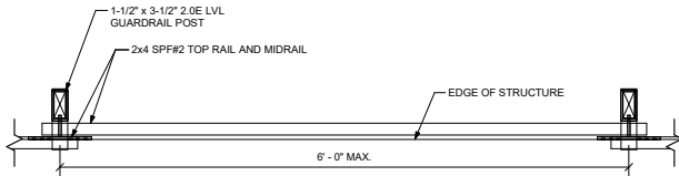
11 MIGHTYRAIL VERTICAL MOUNT EXAMPLE PLAN VIEW S101.2
