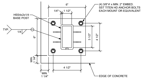
MIGHTYRAIL FLOOR MOUNT TOP SECTION CONCRETE ANCHOR OPTION
