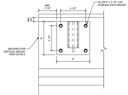
3 MIGHTYRAIL VERTICAL MOUNT FRONT SECTION LAG SCREW OPTION S100.2
