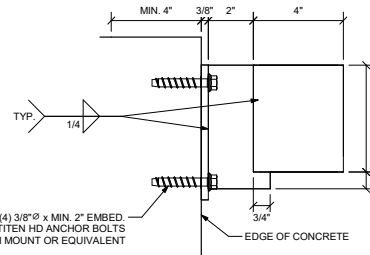
8 MIGHTYRAIL VERTICAL MOUNT SIDE SECTION CONCRETE ANCHOR OPTION S100.1
