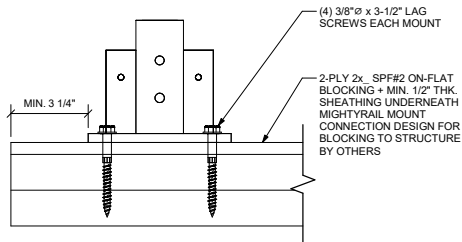
MIGHTYRAIL FLOOR MOUNT FRONT SECTION LAG SCREW OPTION
