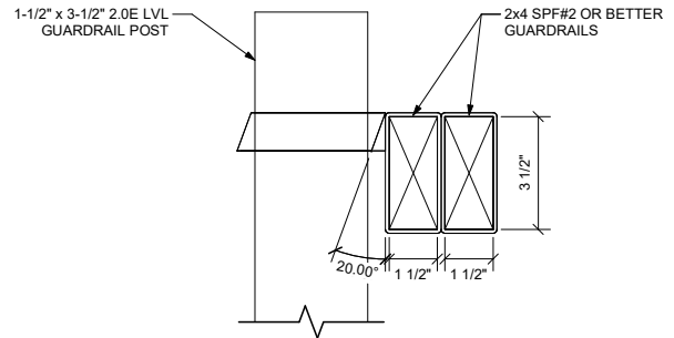
6 MIGHTYRAIL RAILING PIECE SIDE SECTION S101.2
