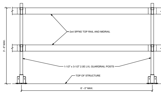
MIGHTYRAIL FLOOR MOUNT EXAMPLE ELEVATION VIEW
