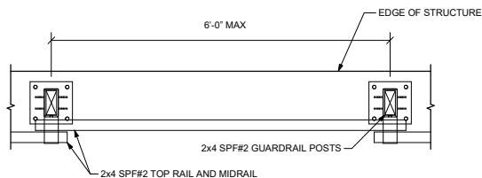
MIGHTYRAIL FLOOR MOUNT EXAMPLE PLAN VIEW
