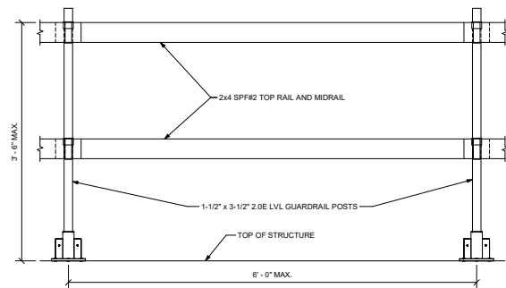
8 MIGHTYRAIL FLOOR MOUNT EXAMPLE ELEVATION VIEW S101.2
