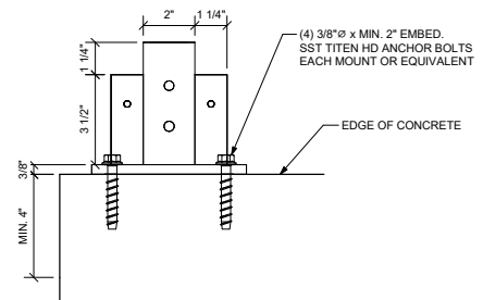
MIGHTYRAIL FLOOR MOUNT FRONT SECTION CONCRETE ANCHOR OPTION
