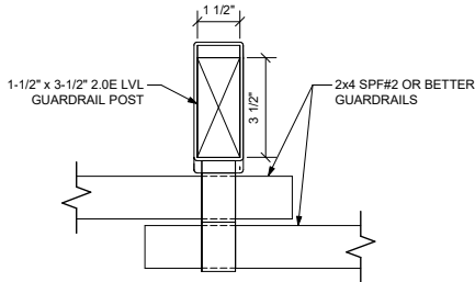
7 MIGHTYRAIL RAILING PIECE TOP SECTION S101.2
