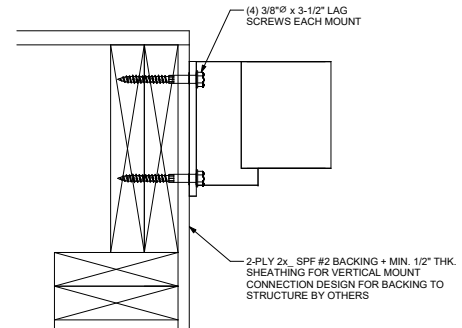
4 MIGHTYRAIL VERTICAL MOUNT SIDE SECTION LAG SCREW OPTION S100.2
