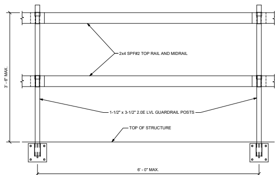
7 MIGHTYRAIL VERTICAL MOUNT EXAMPLE ELEVATION VIEW S101
